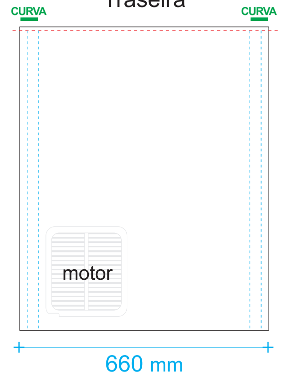
Traseira
